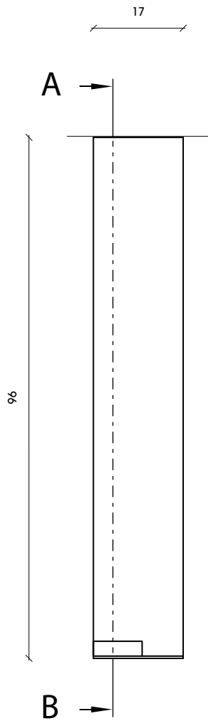
VISTA FRONTAL
